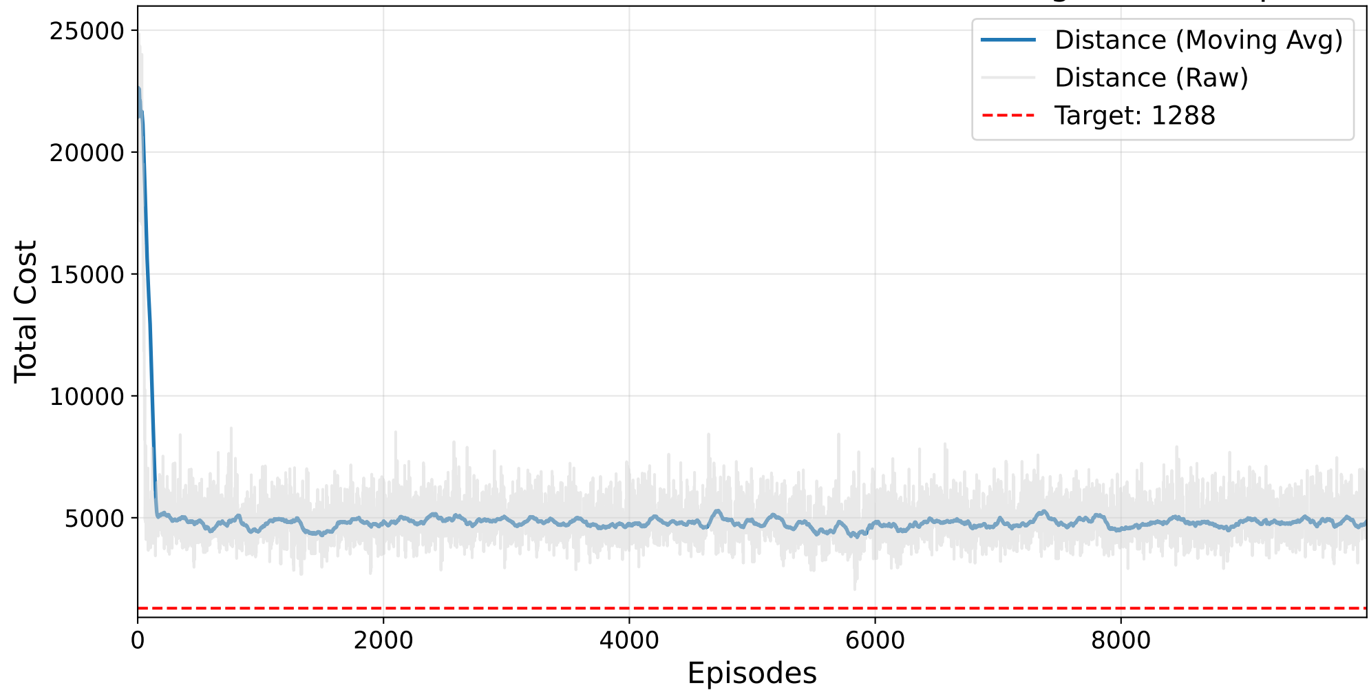
Final HYPERBAND TPE Masked AutoRL-SOP Training - ESC47.sop
